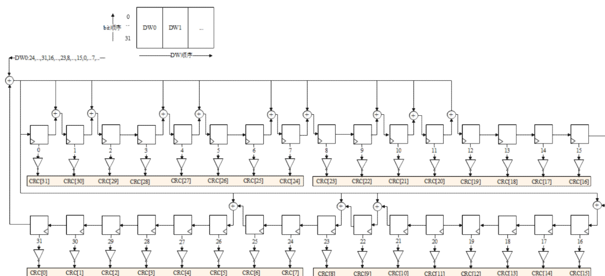
Figure 7 CRC32 Generation Circuit
